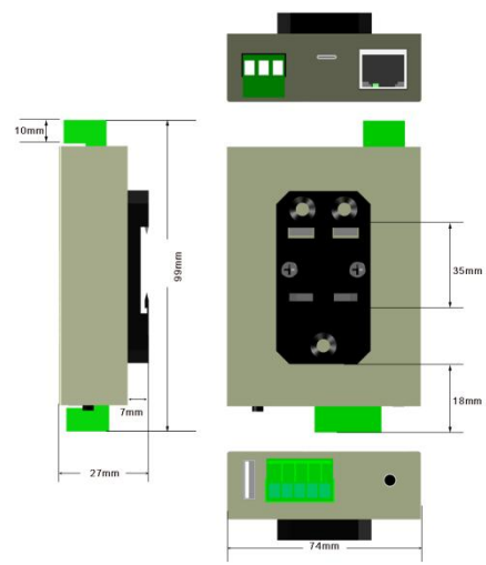
HMI1001-ARM ( back )
