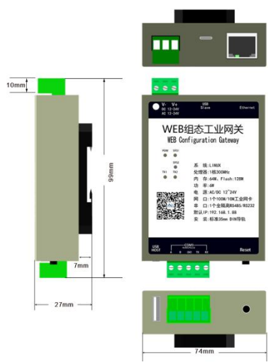
HMI1001-ARM ( front )
